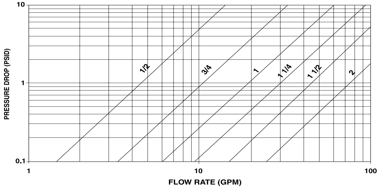
STYLE 2 THREADED BASKET STRAINER PRESSURE DROP - LIQUIDS (SIZES 1/2" - 1-1/2")
