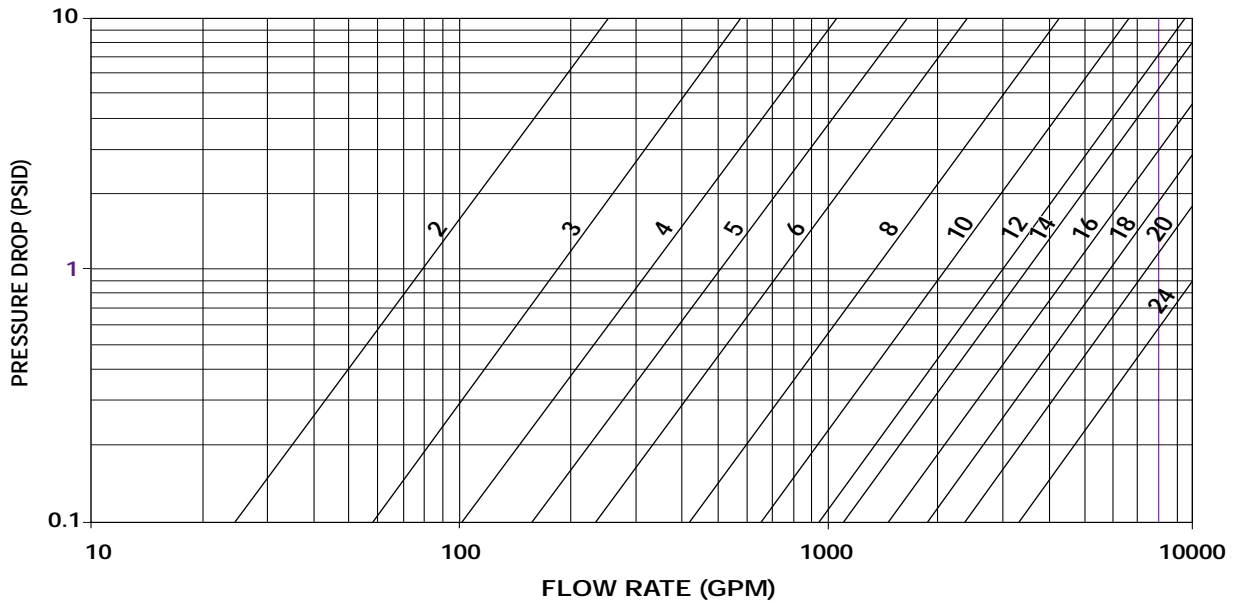
STYLE 2 FLANGED BASKET STRAINER PRESSURE DROP - LIQUIDS (SIZES 2" - 24")
